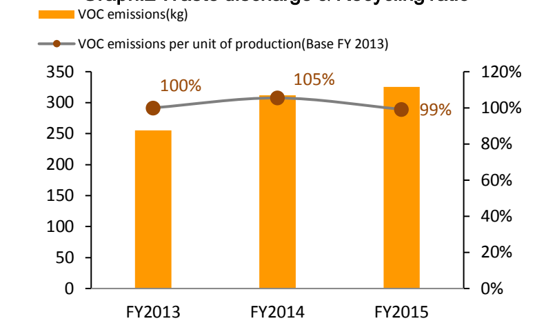
Graph.3 VOC emissions
