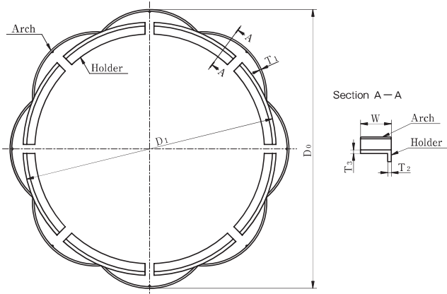
Appendix Table 31 GX- Accessories (10) Lock Ring Holder (PP)
