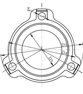
Size 6" and 8"
