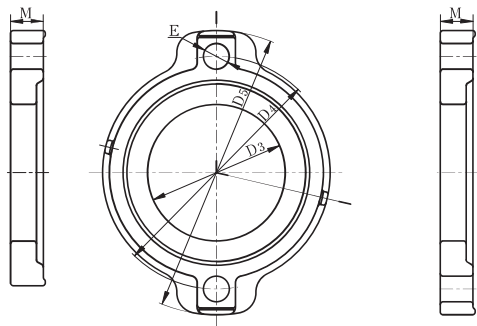
Size 3" and 4"
