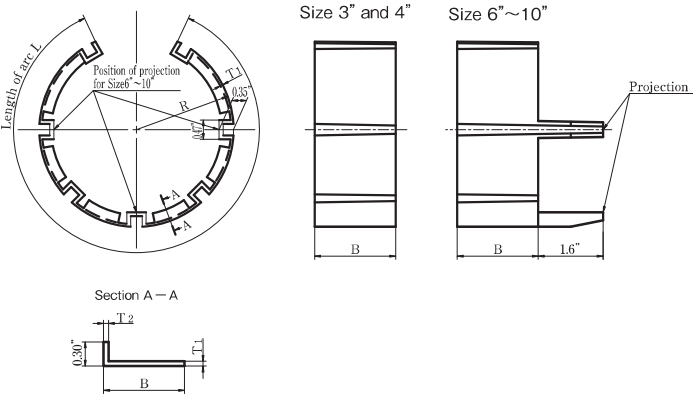
Appendix Table 32 GX- Accessories (11) Liner Board (PA6)
