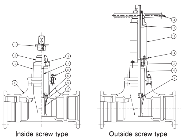
Appendix Table 19 GX-Resilient Seated Gate Valve
