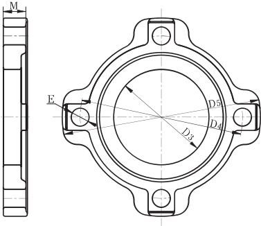
Size 10" ~ 12"
