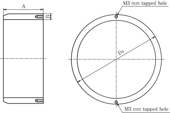
Appendix Table 26 GX- Accessories (5) Liner
